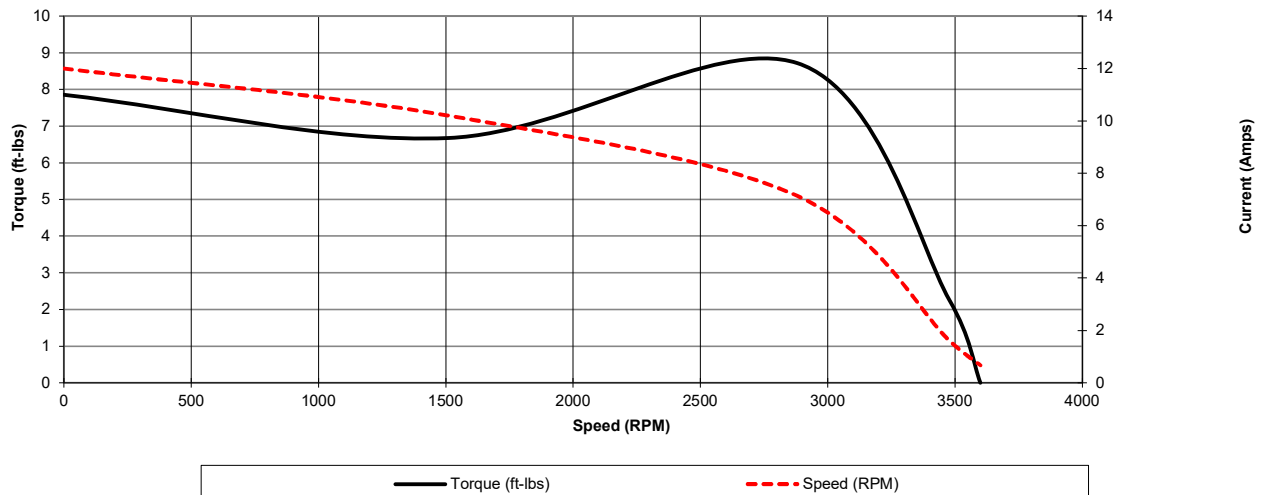
443T - 484T Dual Voltage DOL 31 leads WYE Connection
